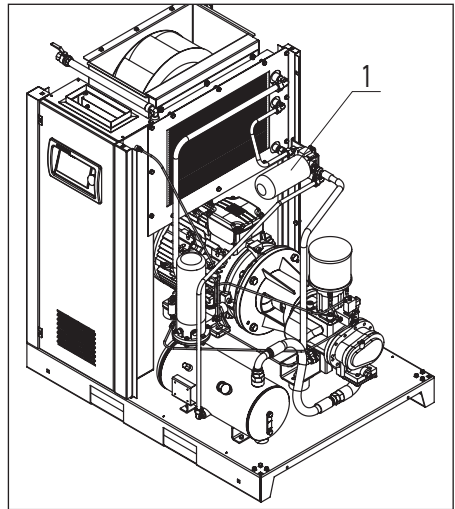
Fig. 5.3.3 Oil replacing DV18 - DV22
