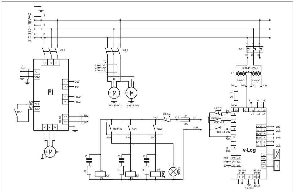
Fig. 2.6.1 Electrical diagram DV11 – DV22
