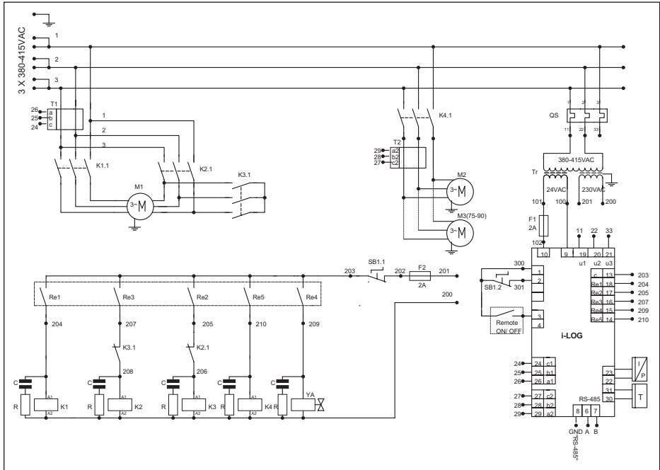
Fig. 2.6 Electrical diagram A75-90
